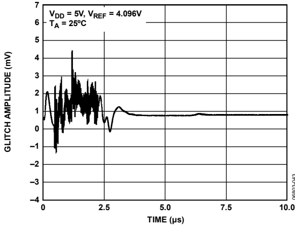
Figure 32. Analog Crosstalk
