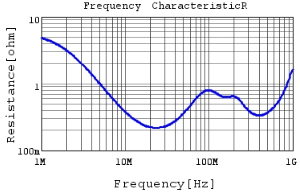
DE11XRA150KA4BH01F R DCOV, 20degC
