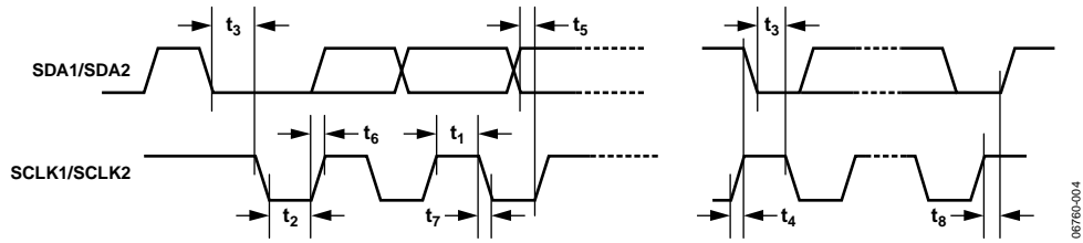
Figure 3. I²C Timing
