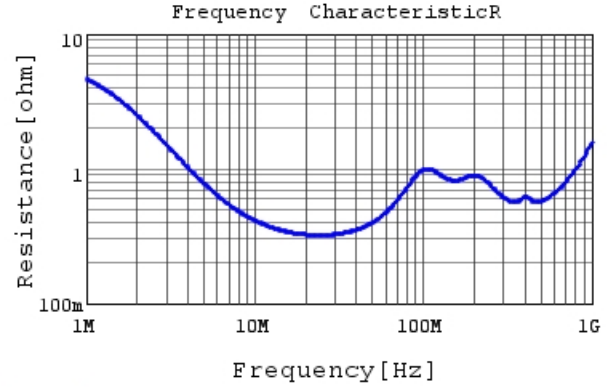
DE11XRA100KJ4BH01F R DC0V, 20degC
