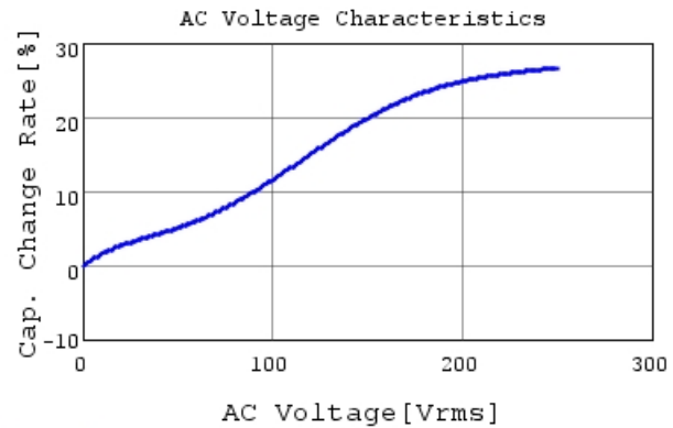
DE1E3RA332MJ4BN01F C-AC Voltage capchange, I
