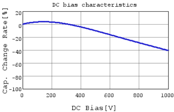
DE1E3RA332MJ4BN01F C-DC bias capchange, 20.0
