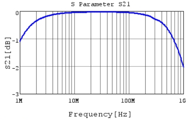
DE1E3RA332MJ4BN01F S21 DCOV, 20degC
