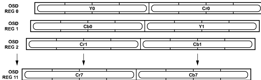
Figure 42. OSD Registers
