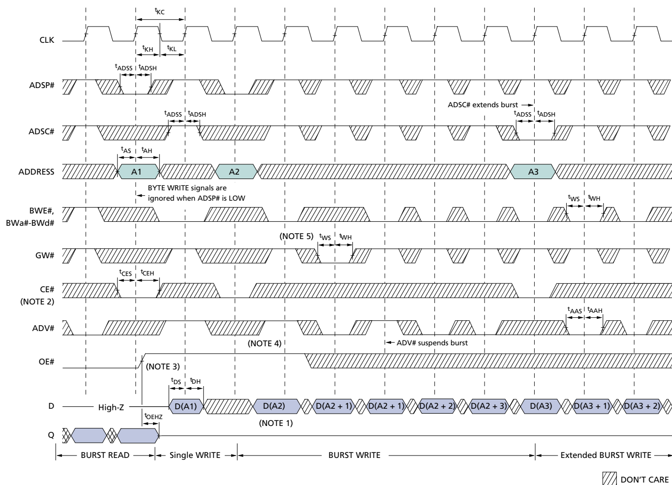
Figure 8: WRITE Timing
