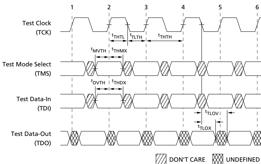
Figure 17: TAP Timing
