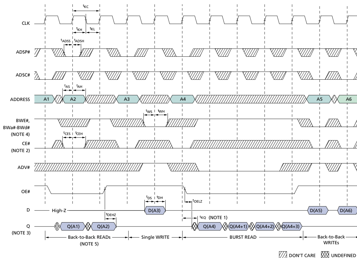
Figure 9: READ/WRITE Timing
