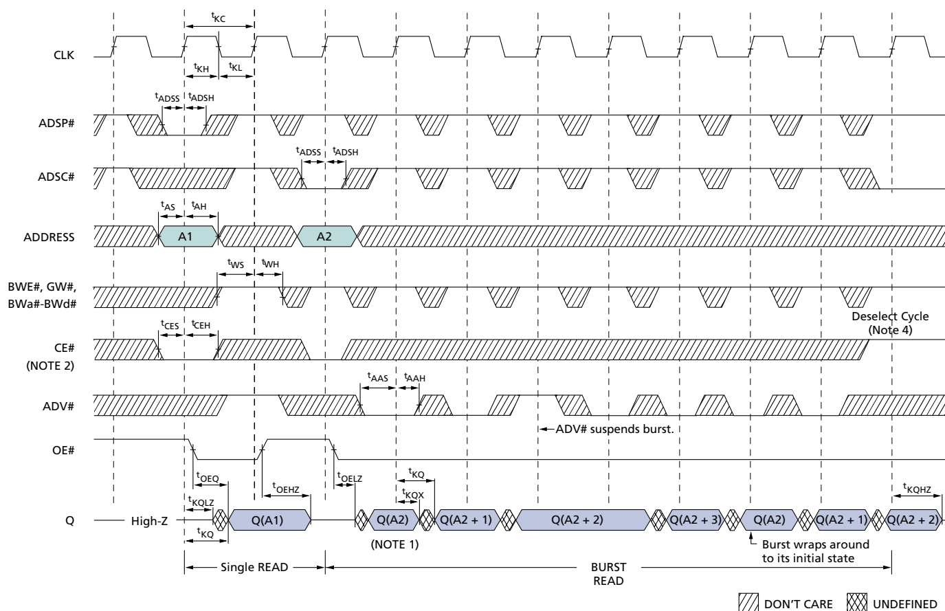
Figure 7: READ Timing
