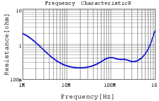
DE11XRA330KN4AH01F R DCOV, 20degC
