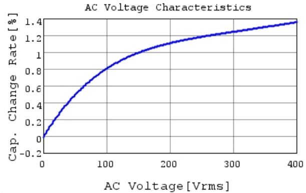
DE11XRA330KN4AH01F C-AC Voltage capchange, I
