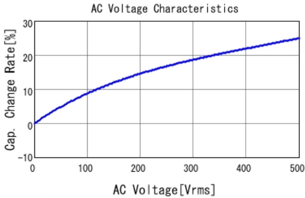
DE1B3RB471KN4AR01F C-AC Voltage capchange, DCOV, 2
