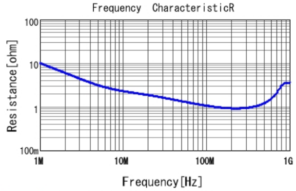
DE1B3RB471KN4AR01F R DCOV, 20degC
