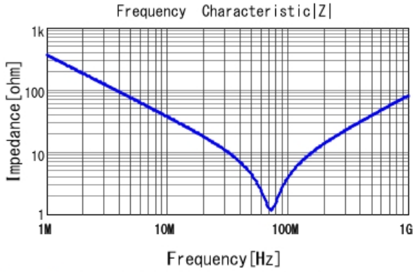
DE1B3RB471KN4AR01F |Z| DCOV, 20degC
