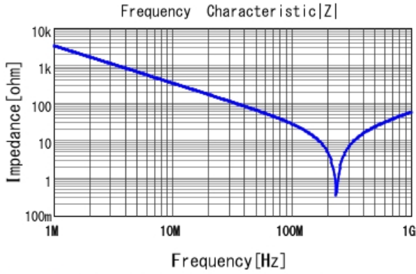
DE21XSA470KN3AT02F |Z| DCOV, 20degC
