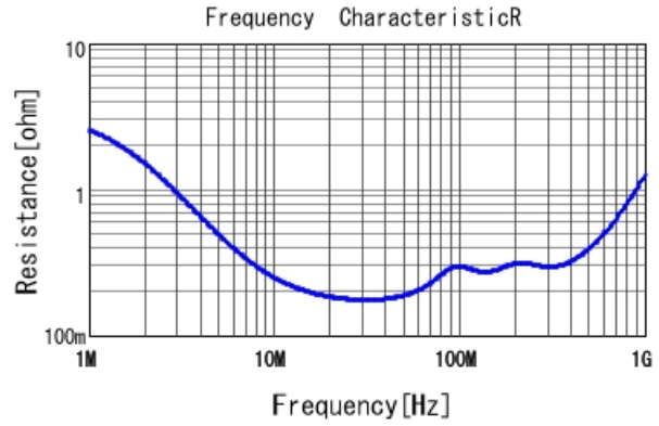
DE21XSA470KN3AT02F R DCOV, 20degC
