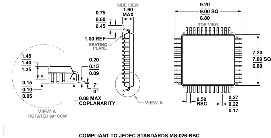
Figure 86. 48-Lead Low Profile Quad Flat Package [LQFP] 7 mm × 7 mm Body (ST-48)
