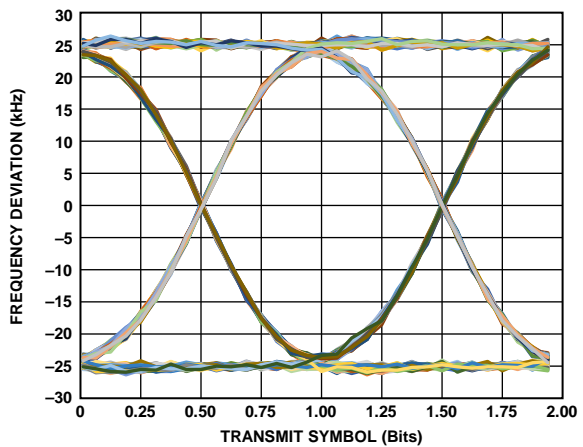
Figure 32. Transmit Eye Diagram, PA2 Output Power = 17 dBm, Configuration 433 MHz/50 kbps, V_{DD} = 3.0 V , T_A = 25^\circ C
