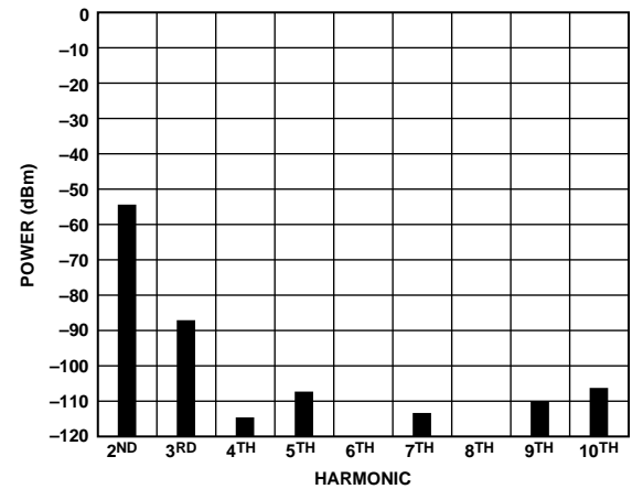
Figure 31. Conductive Harmonic Emission Level, PA1 Output Power = 10 dBm, RF Frequency = 433.92 MHz, V_{DD} = 3.0 V , T_A = 25^\circ C
