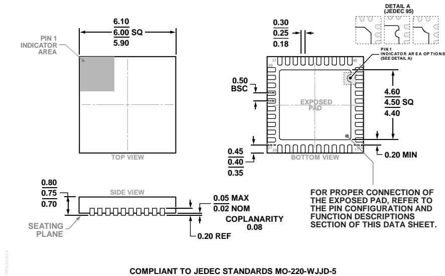
Figure 85. 40-Lead Lead Frame Chip Scale Package [LFCSP] 6 mm × 6 mm Body and 0.75 mm Package Height (CP-40-17)
