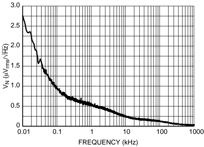
Figure 31. Output Voltage Noise, 1.2 V Version, V_{IN} = 2.2\text{ V}
