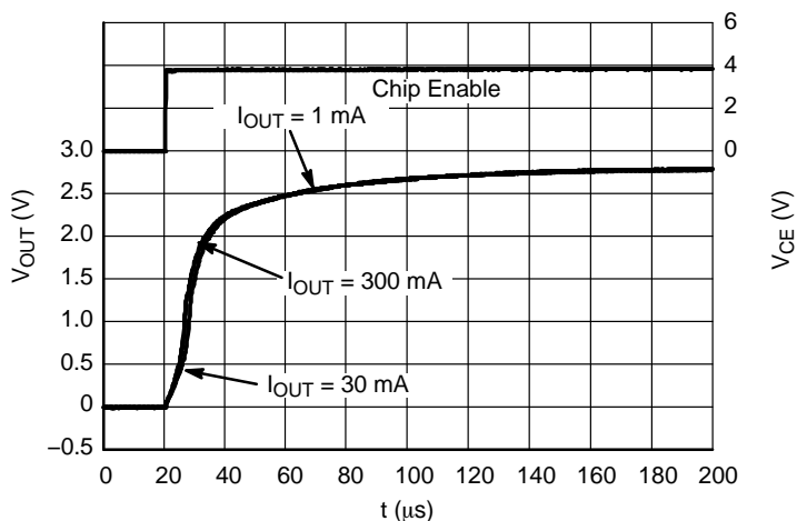
Figure 53. Start-up, 2.8 V Version, V_{IN} = 3.8 V
