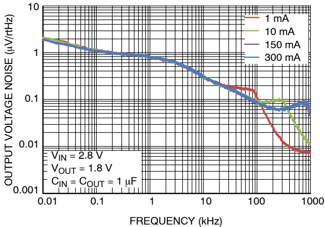
Figure 24. Output Voltage Noise Spectral Density for VOUT = 2.8 V, COUT = 1 uF
