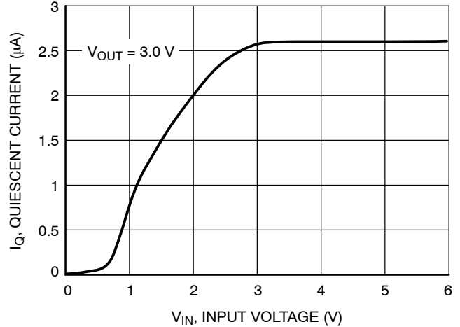
Figure 4. Quiescent Current versus Input Voltage
