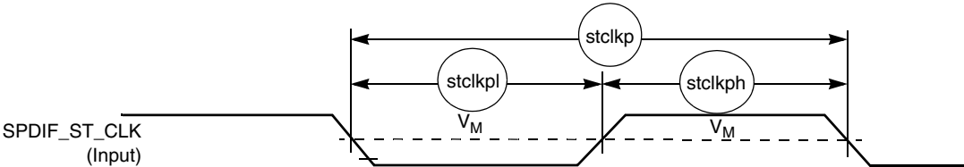
Figure 44. STCLK Timing Diagram
