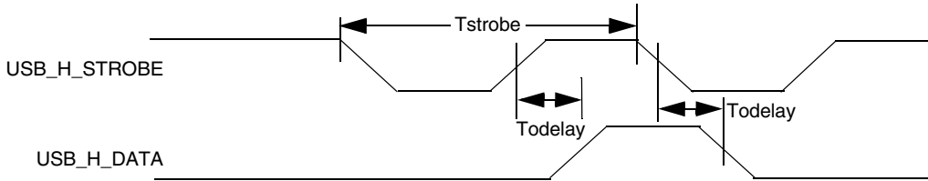
Figure 53. USB HSIC Transmit Waveform
