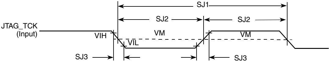
Figure 39. Test Clock Input Timing Diagram
