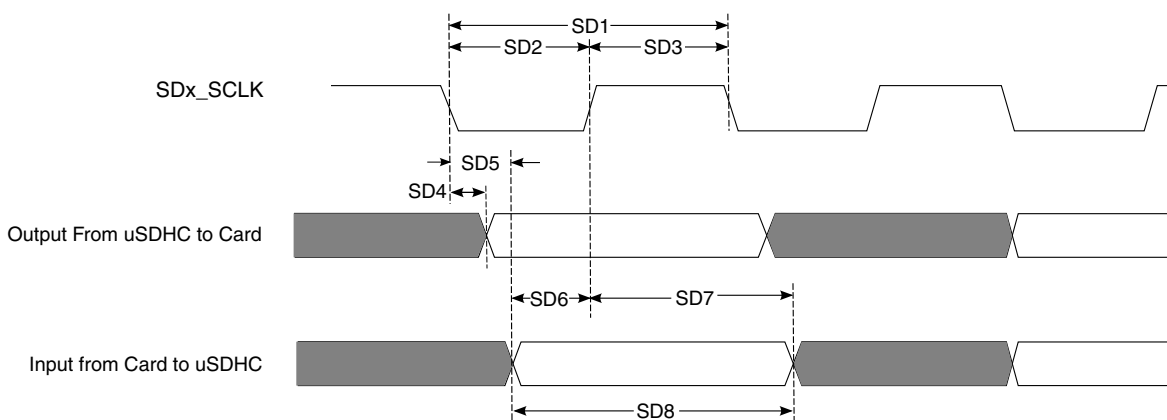
Figure 35. SDR50/SDR104 Timing
