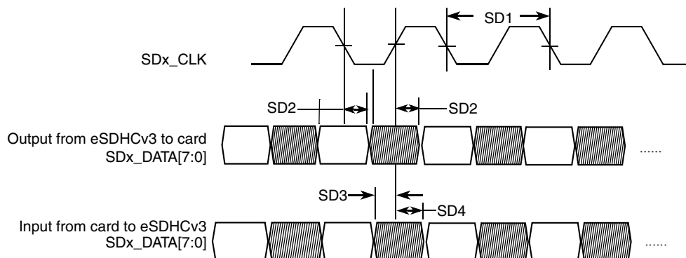
Figure 34. eMMC4.4/4.41 Timing
