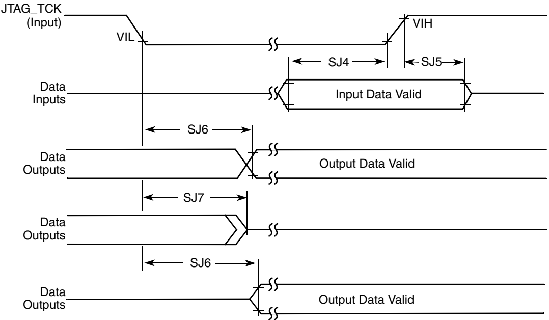
Figure 40. Boundary Scan (JTAG) Timing Diagram
