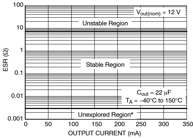
Figure 15. ESR Stability Region vs. Output Current
