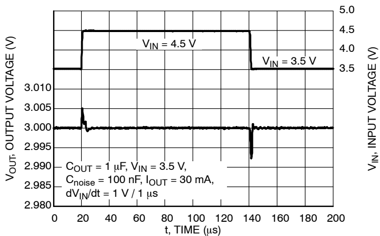
Figure 32. Line Transient Response, V_{\text{OUT}} = 3.0 \text{ V} , C_{\text{OUT}} = 1 \mu\text{F} , I_{\text{OUT}} = 30 \text{ mA}
