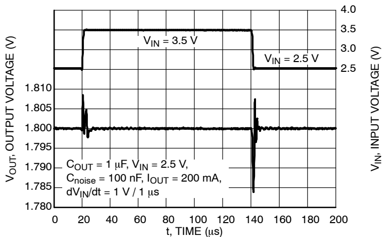
Figure 31. Line Transient Response, V_{\text{OUT}} = 1.8 \text{ V} , C_{\text{OUT}} = 1 \mu\text{F} , I_{\text{OUT}} = 200 \text{ mA}
