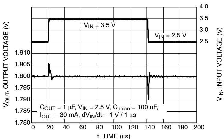
Figure 30. Line Transient Response, V_{\text{OUT}} = 1.8 \text{ V} , C_{\text{OUT}} = 1 \mu\text{F} , I_{\text{OUT}} = 30 \text{ mA}
