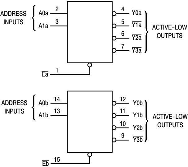
Figure 1. Logic Diagram
