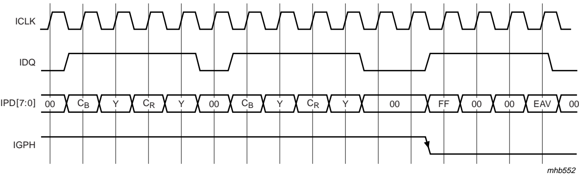
Fig 44. Output timing I port for serial 8-bit data at end of a line (ICODE = 1)
