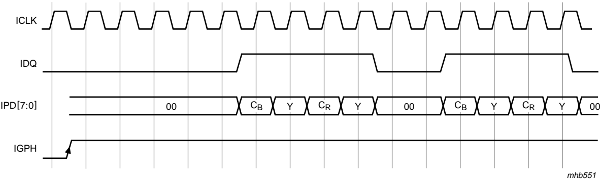
Fig 43. Output timing I port for serial 8-bit data at start of a line (ICODE = 0)
