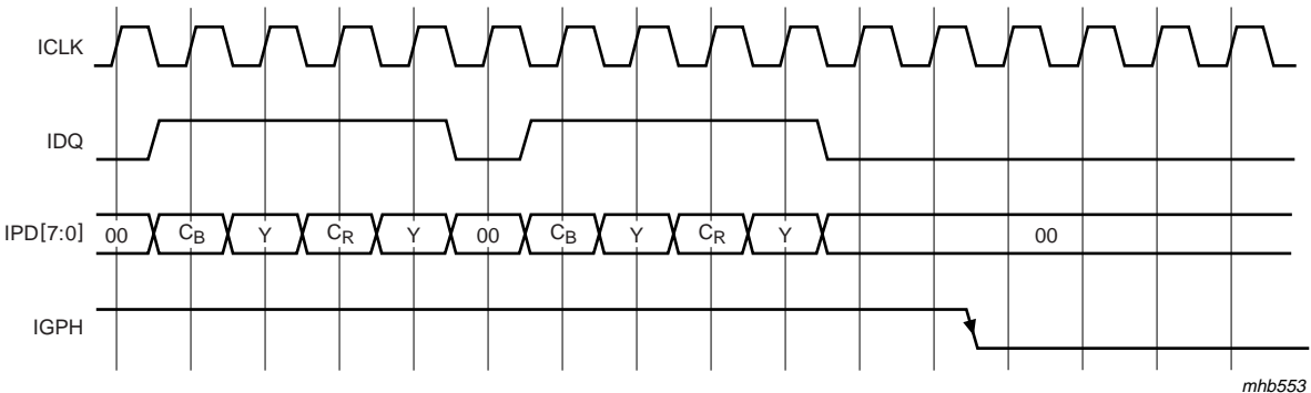
Fig 45. Output timing I port for serial 8-bit data at end of a line (ICODE = 0)
