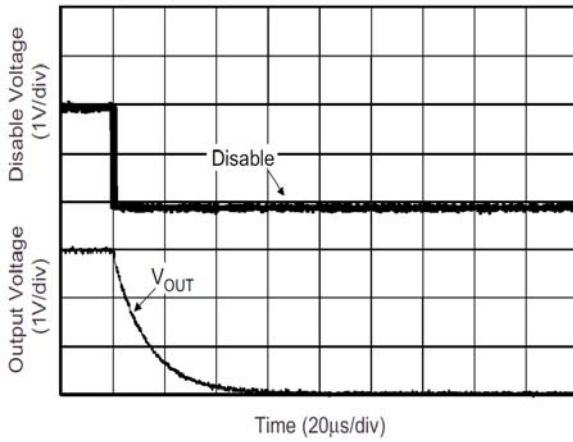
Figure 23. Shutdown Delay
