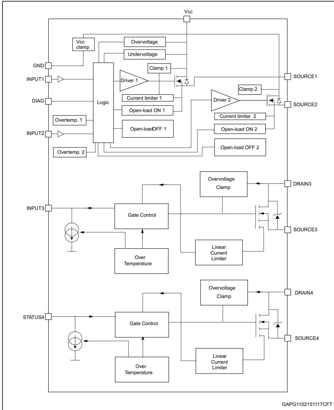
Figure 1. Block diagram
