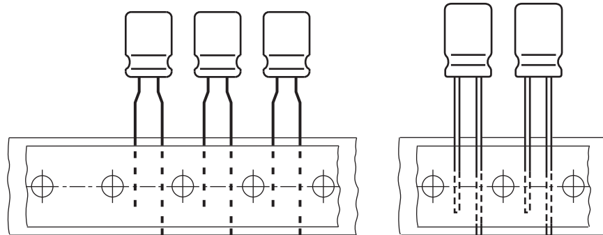
Pitch F = 2.5 mm Case Ø D = 4 mm to 6.3 mm
