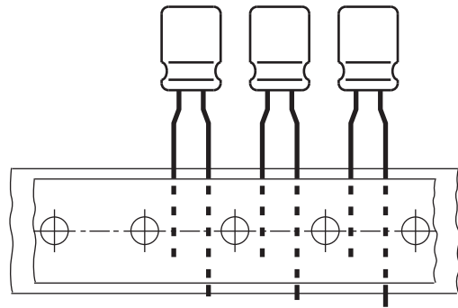
Case Ø D = 4 mm to 6.3 mm; pitch F = 5 mm
