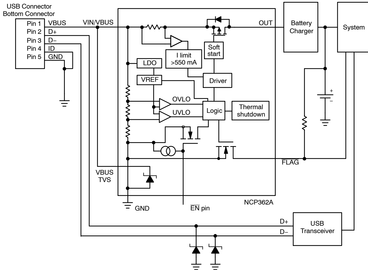
Figure 1. Typical Application Circuit with Wall Adapter / V_{\text{BUS}} TVS Protection (NCP362A)
