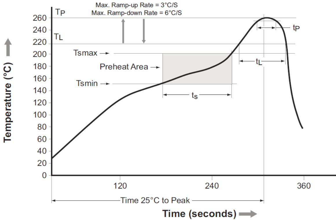
Figure 11. Reflow Profile
