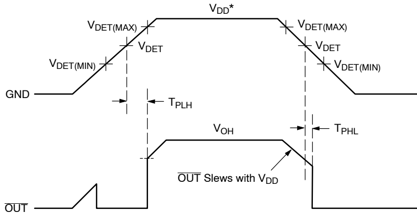
Figure 3. Timing Diagram
