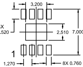
RECOMMENDED MOUNTING FOOTPRINT*
