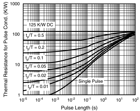
Fig. 7 - Thermal Response
