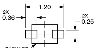
PACKAGE OUTLINE DIMENSIONS: MILLIMETERS
