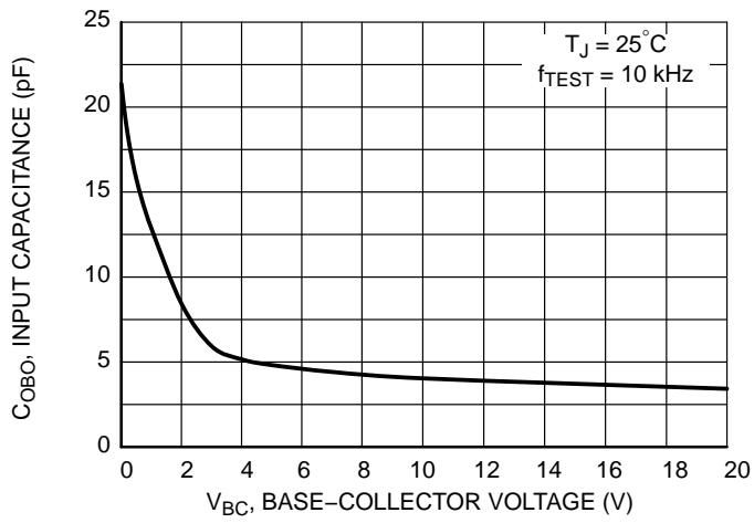
Figure 7. Output Capacitance
