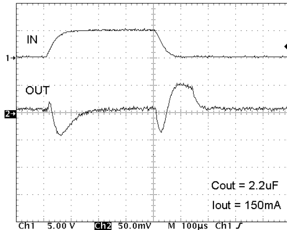
Figure 18. Line Transient ( OUT = 3.3\text{ V} )
