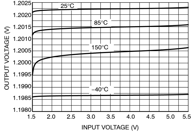
Figure 22. Line Regulation, V_{OUT} = 1.2 V
