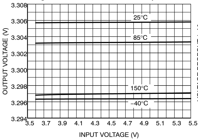
Figure 23. Line Regulation, V_{OUT} = 3.3 V
