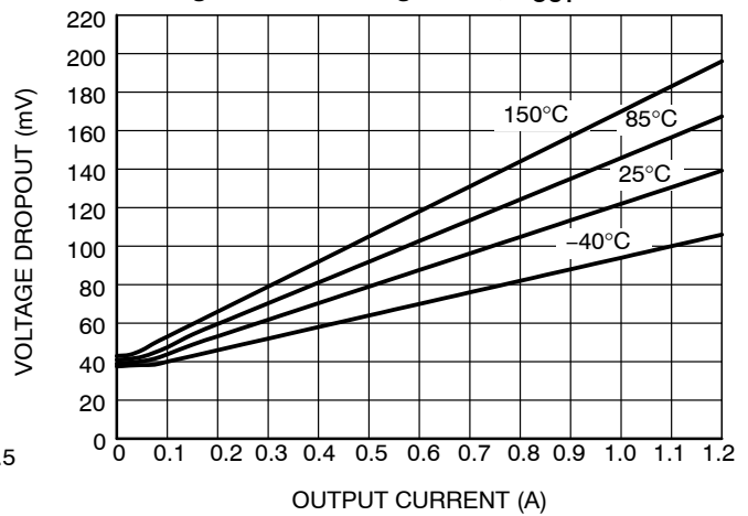
Figure 24. Dropout Voltage vs. Output Current, V_{OUT} = 3.3 V
