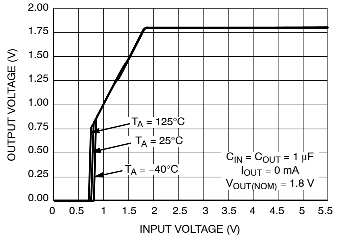
Figure 16. Output Voltage vs. Input Voltage V OUT = 1.8 V
