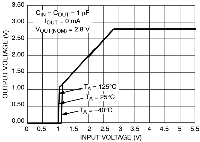
Figure 17. Output Voltage vs. Input Voltage V OUT = 2.8 V
