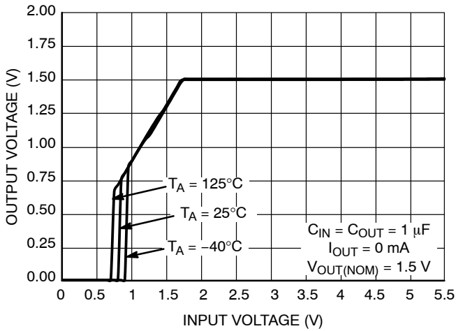
Figure 15. Output Voltage vs. Input Voltage V OUT = 1.5 V
