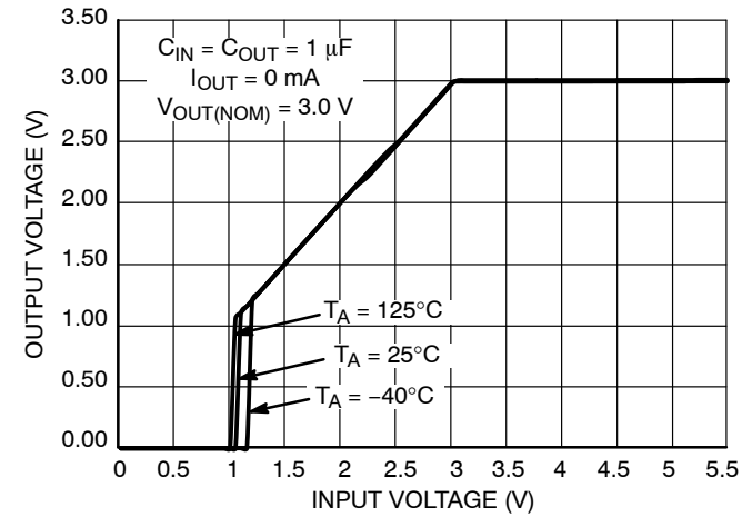
Figure 18. Output Voltage vs. Input Voltage V OUT = 3.0 V
