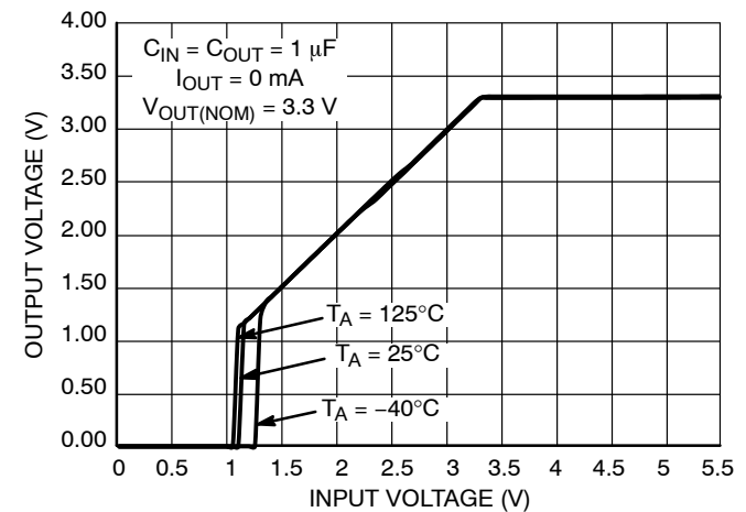
Figure 20. Output Voltage vs. Input Voltage V OUT = 3.3 V
