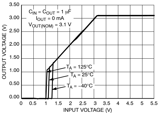
Figure 19. Output Voltage vs. Input Voltage V OUT = 3.1 V
