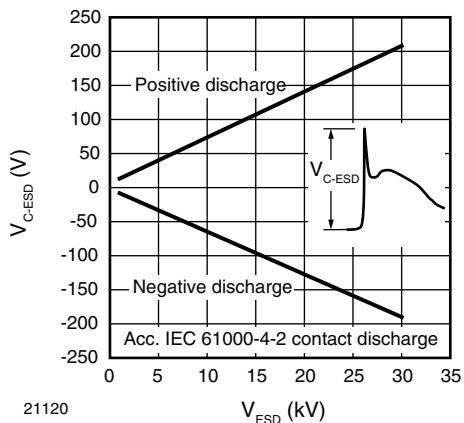
21120 Fig. 9 - Typical Peak Clamping Voltage at ESD Contact Discharge (acc. IEC 61000-4-2)
