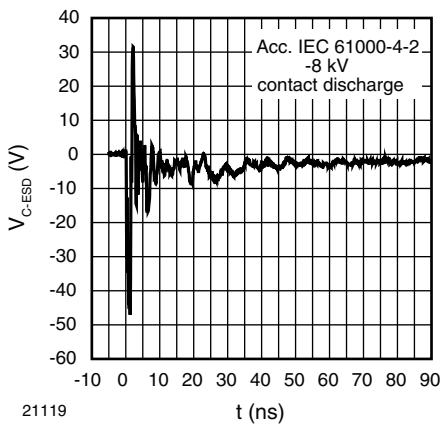
21119 Fig. 8 - Typical Clamping Performance at - 8 kV Contact Discharge (acc. IEC 61000-4-2)
