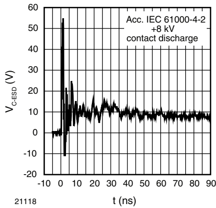
21118 Fig. 7 - Typical Clamping Performance at + 8 kV Contact Discharge (acc. IEC 61000-4-2)
