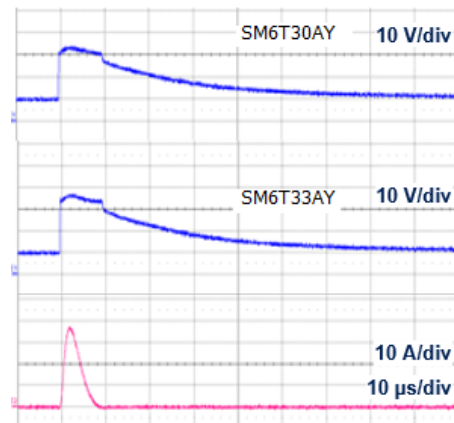
Figure 14. ISO7637-2 pulse 2a: Vs = +112 V with 12 V battery
