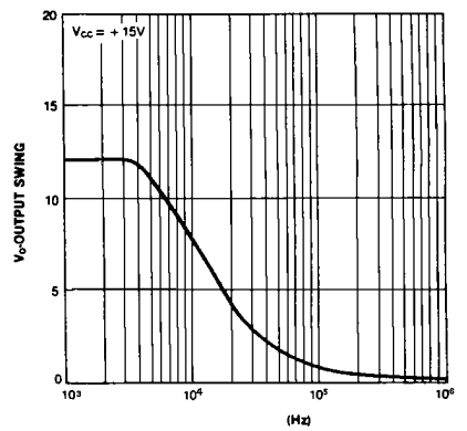
Figure 4. Large Signal Output Swing vs Frequency
