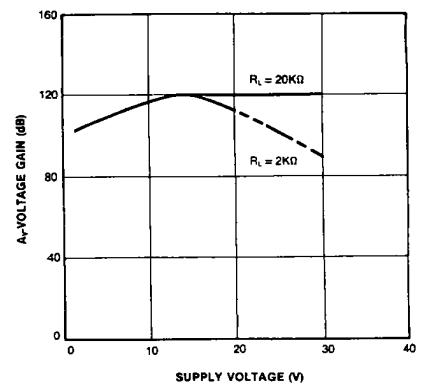
Figure 2. Voltage Gain vs Supply Voltage
