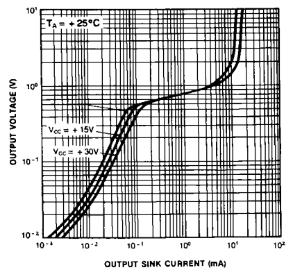
Figure 6. Output Characteristics vs Current Sinking
