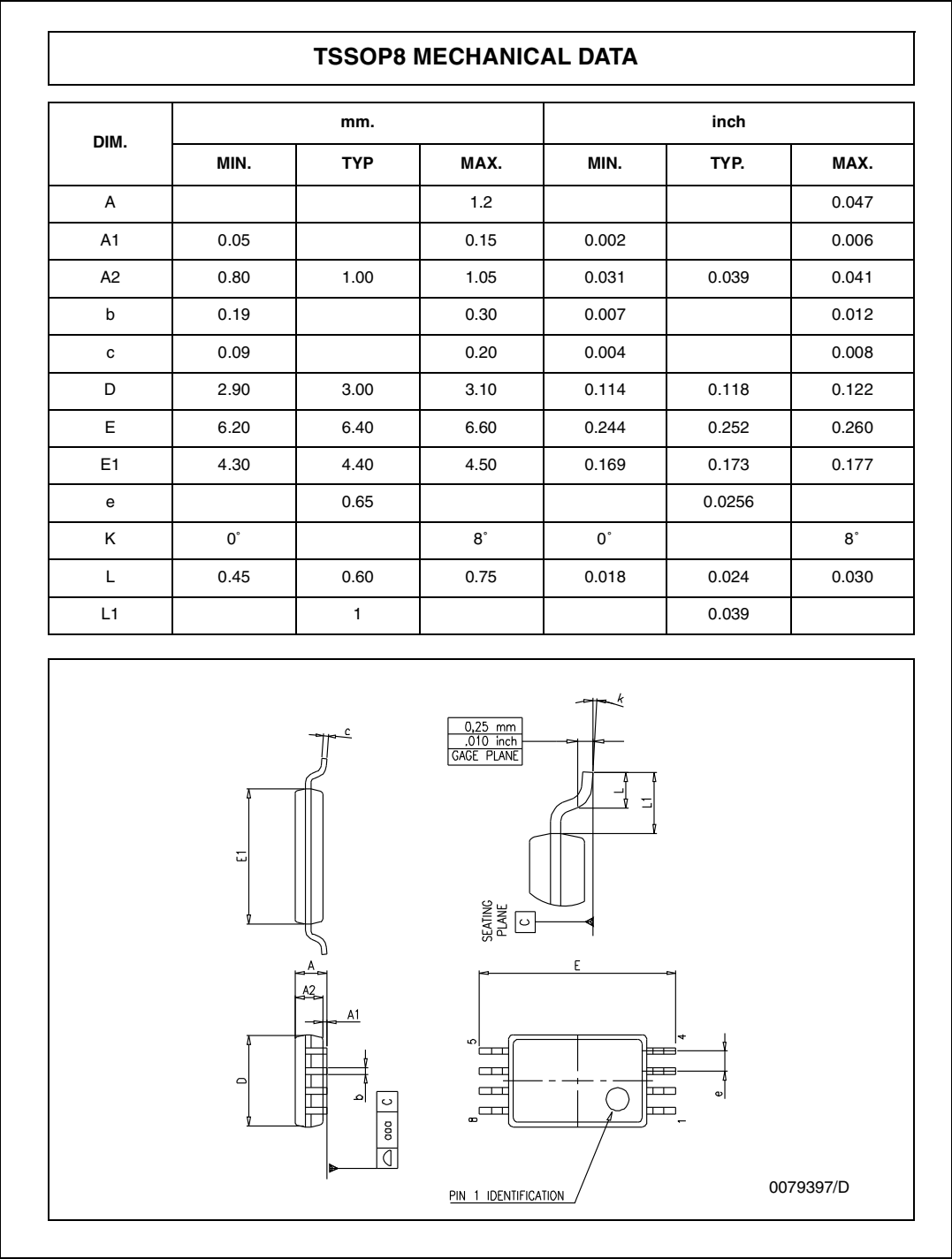
Figure 10. TSSOP8 package
