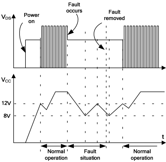
Figure 17. Pulse-Width-Modulation Circuit
