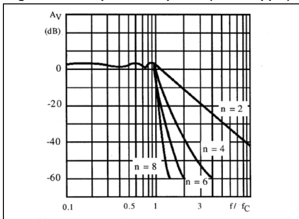
Figure 12. Amplitude response ( \pm 1 dB ripple)
