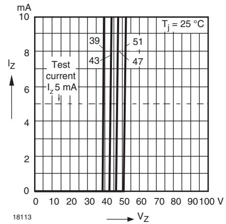
Fig. 14 - Breakdown Characteristics
