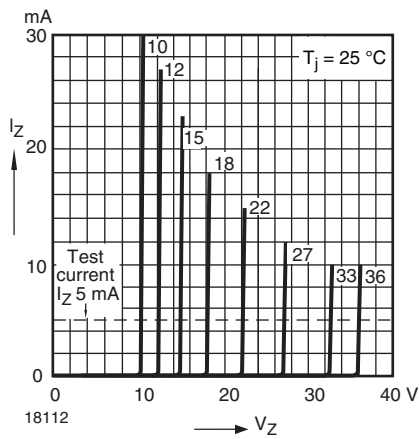
Fig. 13 - Breakdown Characteristics
