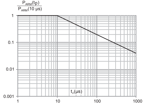
Figure 6. Normalized avalanche power derating versus pulse duration ( T_j = 125^{\circ}C )
