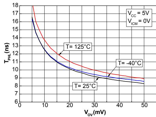
Figure 17. Propagation delay vs. overdrive with negative transition, V_{\text{CC}} = 5\text{V}
