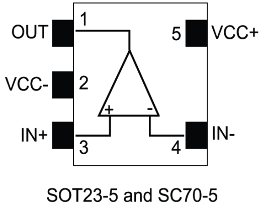
Figure 1. Pin configuration
