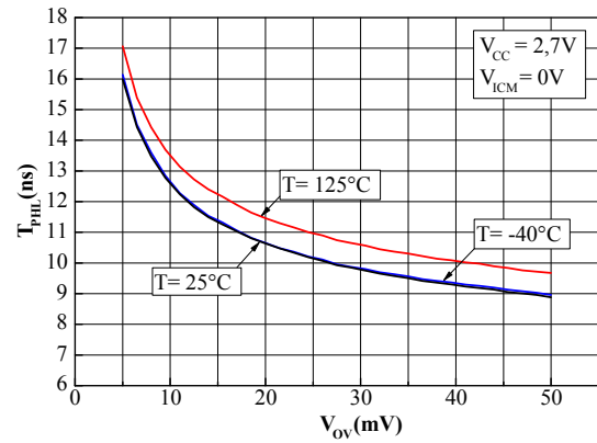
Figure 15. Propagation delay vs. overdrive with negative transition, V_{\text{CC}} = 2.7\text{V}
