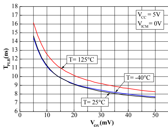
Figure 18. Propagation delay vs. overdrive with positive transition, V_{\text{CC}} = 5\text{V}
