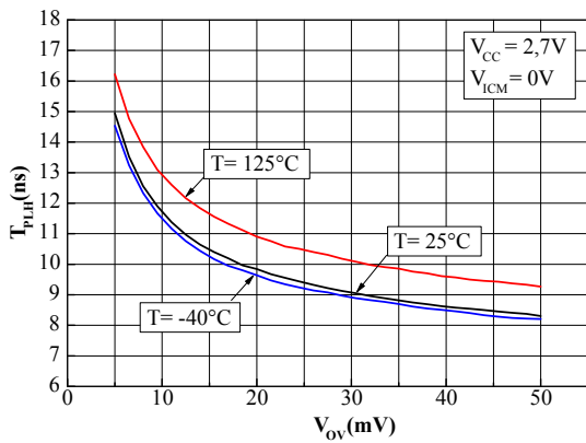
Figure 16. Propagation delay vs. overdrive with positive transition, V_{\text{CC}} = 2.7\text{V}
