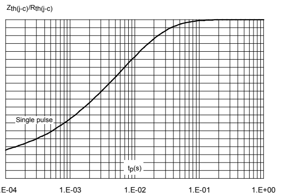
Figure 4. Relative variation of Z_{th(j-c)} versus pulse duration
