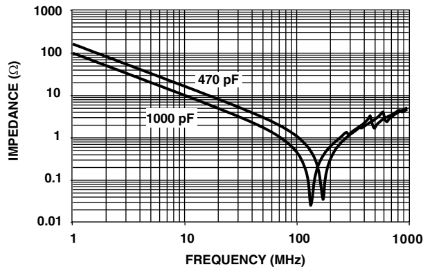
IMPEDANCE VS. FREQUENCY OF 1206 NP0 HVArc Guard®
