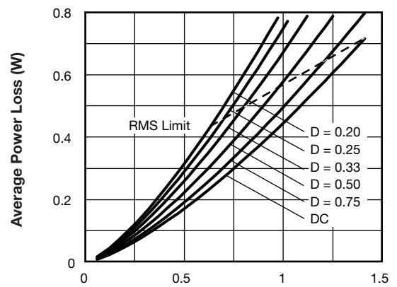
94614_05 Average Forward Current - I F(AV) (A) Fig. 5 - Forward Power Loss Characteristics
