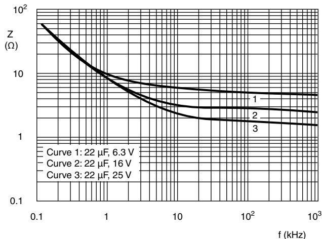
Fig.8 Typical impedance as a function of frequency at 20 ^{\circ}C
