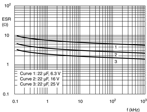
Fig.6 Typical ESR as a function of frequency at 20 ^{\circ}C
