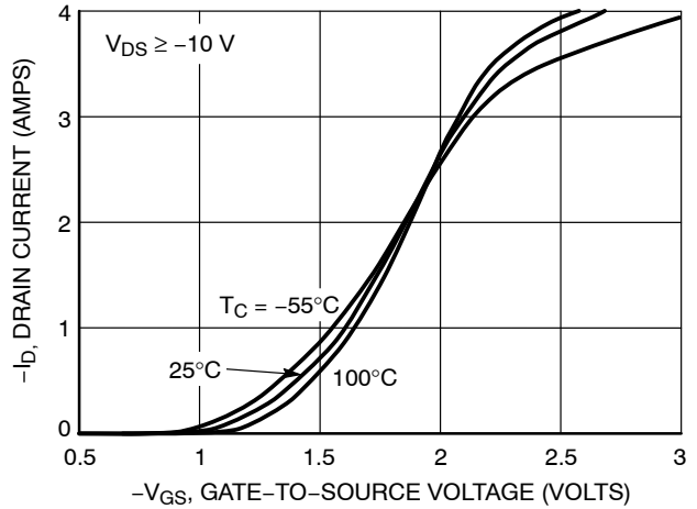
Figure 12. Transfer Characteristics
