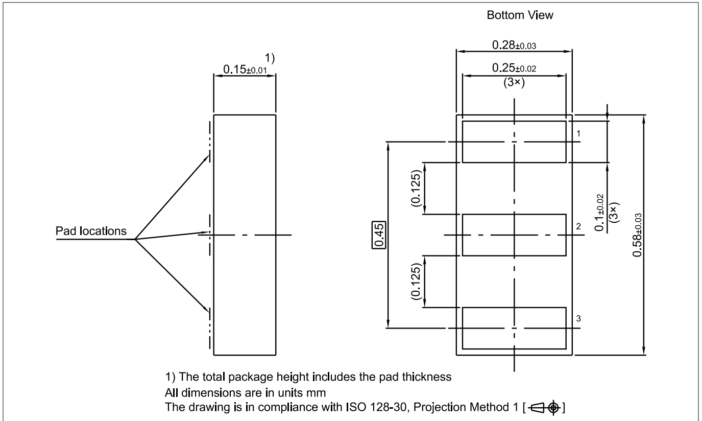
Figure 12 WLL-3-1 package
