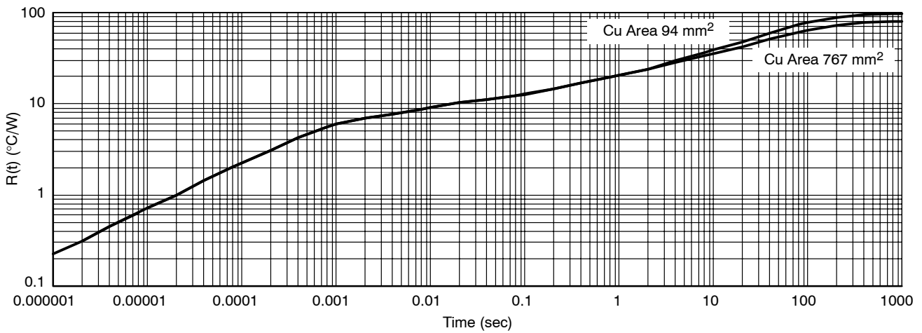
Figure 24. SOIC 16-Lead Single Pulse Heating Curve
