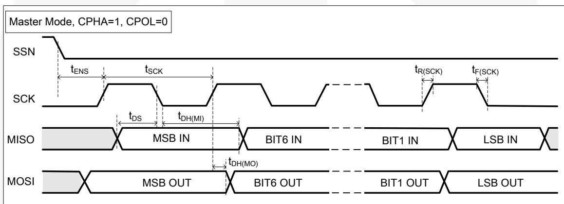
Figure 7. SPI Timing Diagram – Master Mode
