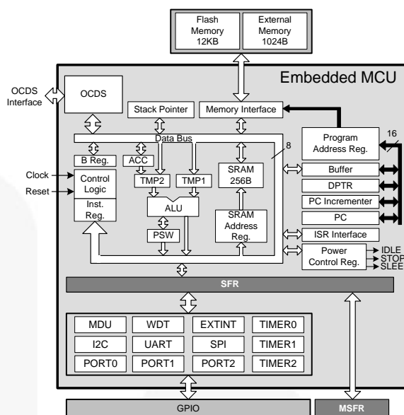
Figure 20. Embedded MCU Block Diagram
