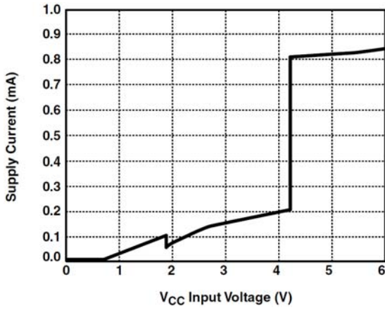
Figure 1. V CC Supply Current vs. Voltage
